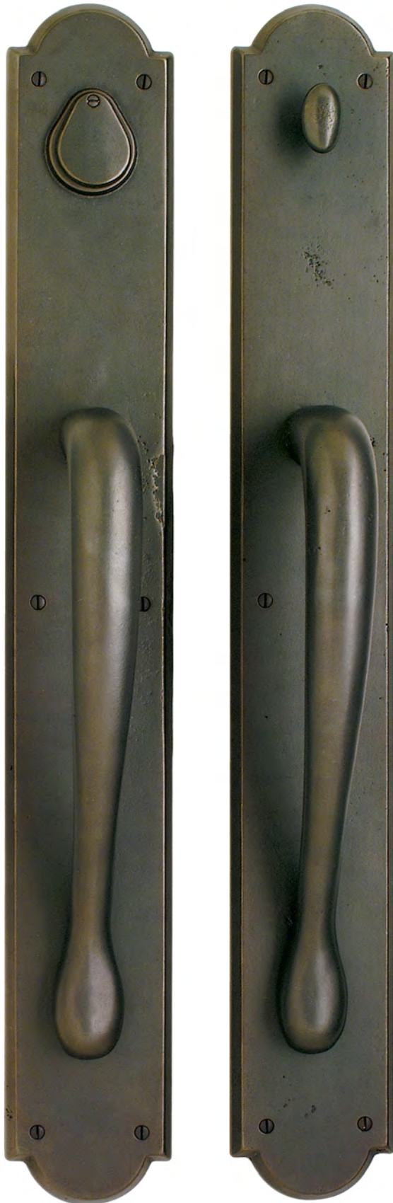
ESCUTCHEON 3 1/2" x 26" FUNCTION PULL/PULL DEADBOLT GRIP G614 12" GOOSENECK PATINA SILICON BRONZE, DARK PART # G781/G782
